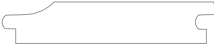
PLANKING 93884 3/4" X 3 7/8" LAYS 3 1/2"
