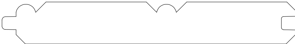
PLANKING 9525_11 3/4" X 5 1/4" LAYS 5"
